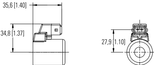
Y0 AMP Junior Timer integrated connector
