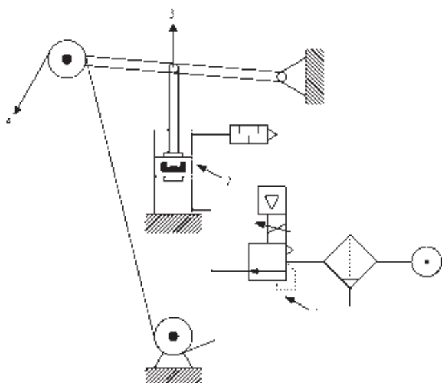
CYLINDER IN THRUST
