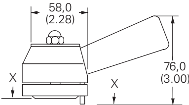
MRV2-16-D/L Models
