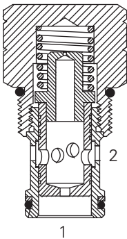
Sectional View
