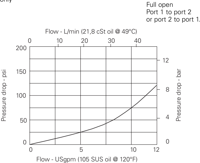
Pressure Drop Curve Cartridge only
