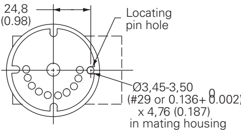
MRV2-16-D Models
