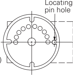
MRV2-16-L Models
