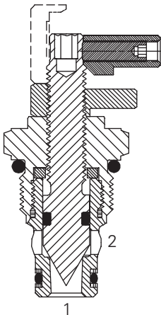
Sectional View
