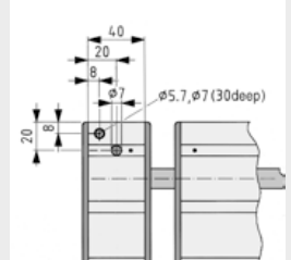
Recommended arrangement for a fixing or mounting hole.
