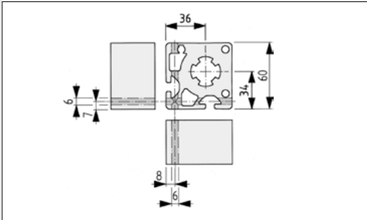
Ball-bush block guides, size 60x60, Shaft D25
