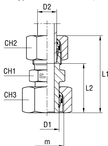
Type: 1053...4 B4 Ring
