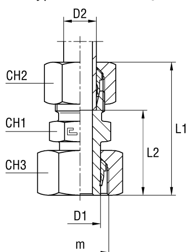
Type: 1053.. B3 Ring
