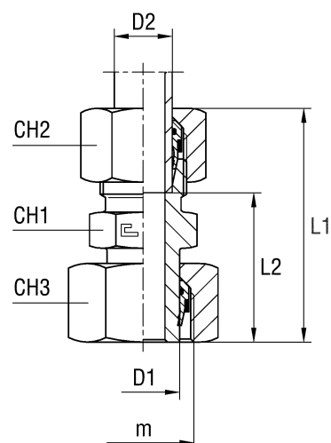
Type: 1054...4 B4 Ring
